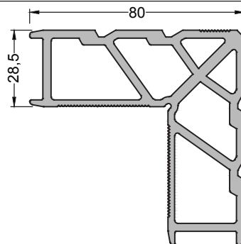
1285 ( 3,511 kg/mt ) L285 CORNER JOINT
