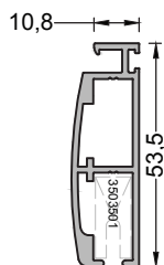
380-4003 ( 0,661 kg/mt ) S72S03 FLYSCREEN VENT PR.
