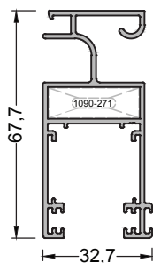
380-4006 ( 1,003 kg/mt ) SLA-S01 FLYSCREEN VENT PR.
