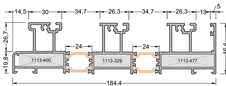
320-1302 ( 4,229 kg/mt ) SAT120 F05 FRAME PROFILE
