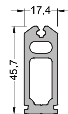
800-345 ( 0,319 kg/mt ) G345 GLAZING BEAD
