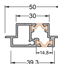
320-6002 ( 0,760 kg/mt ) SAT120A01 ADAPTER PROFILE
