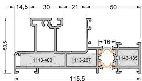
320-1102 ( 2,542 kg/mt ) SAT120 F10 FRAME PROFILE
