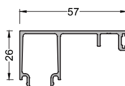
320-6008 ( 0,570 kg/mt ) SAT120C02 ADAPTER PROFILE
