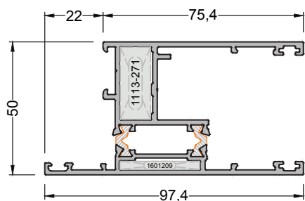
320-2101 ( 1,900 kg/mt ) SAT120V01 VENT PROFILE
