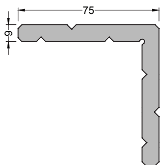
1090 ( 3,284 kg/mt ) L090 CORNER JOINT
