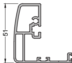
320-6005 ( 1,059 kg/mt ) SAT120A04 ADAPTER PROFILE
