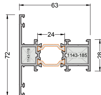
263-2101 ( 1,546 kg/mt ) WAT63M01 MULLION PROFILE
