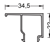
800-345 ( 0,319 kg/mt ) G345 GLAZING BEAD
