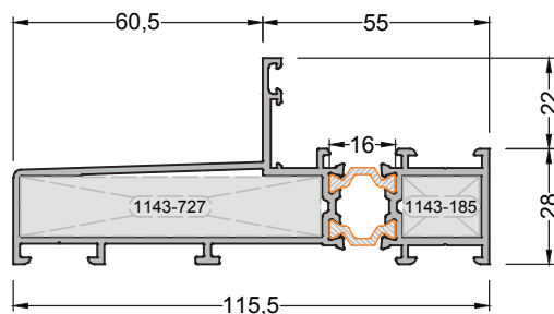
320-1404 ( 1,926 kg/mt ) SAT120F09 FRAME PROFILE
