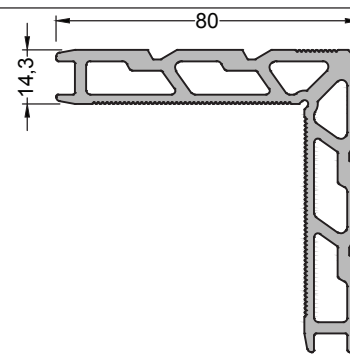
1143 ( 2,867 kg/mt ) L143 CORNER JOINT
