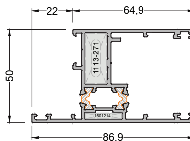
320-2102 ( 1,689 kg/mt ) SAT120V02 VENT PROFILE
