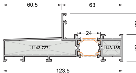
320-1403 ( 1,969 kg/mt ) SAT120F08 FRAME PROFILE
