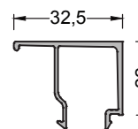
800-325 ( 0,313 kg/mt ) G325 GLAZING BEAD
