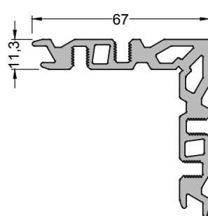
1113 ( 2,188 kg/mt ) L113 CORNER JOINT
