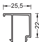
800-255 ( 0,285 kg/mt ) G255 GLAZING BEAD
