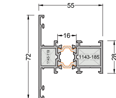
255-2101 ( 1,505 kg/mt ) WAT55M01 MULLION PROFILE
