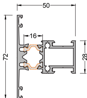
320-3101 ( 1,347 kg/mt ) SAT120M01 MULLION PROFILE
