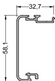
320-6009 ( 0,522 kg/mt ) SAT120C03 ADAPTER PROFILE
