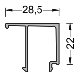
800-285 ( 0,296 kg/mt ) G285 GLAZING BEAD
