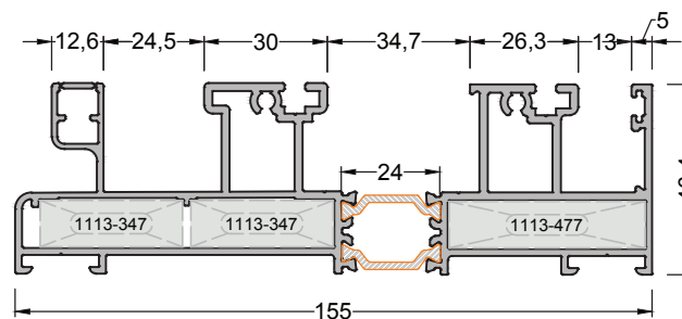
320-1203 ( 3,351 kg/mt ) SAT120 F11 FRAME PROFILE
